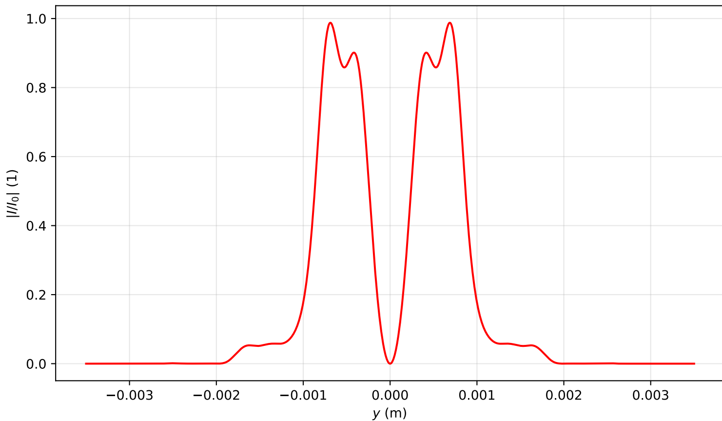
Intensity profile I(x=0, y, z=1.513)/I_0 , P_{in}=7.0P_{cr} , artificial time
